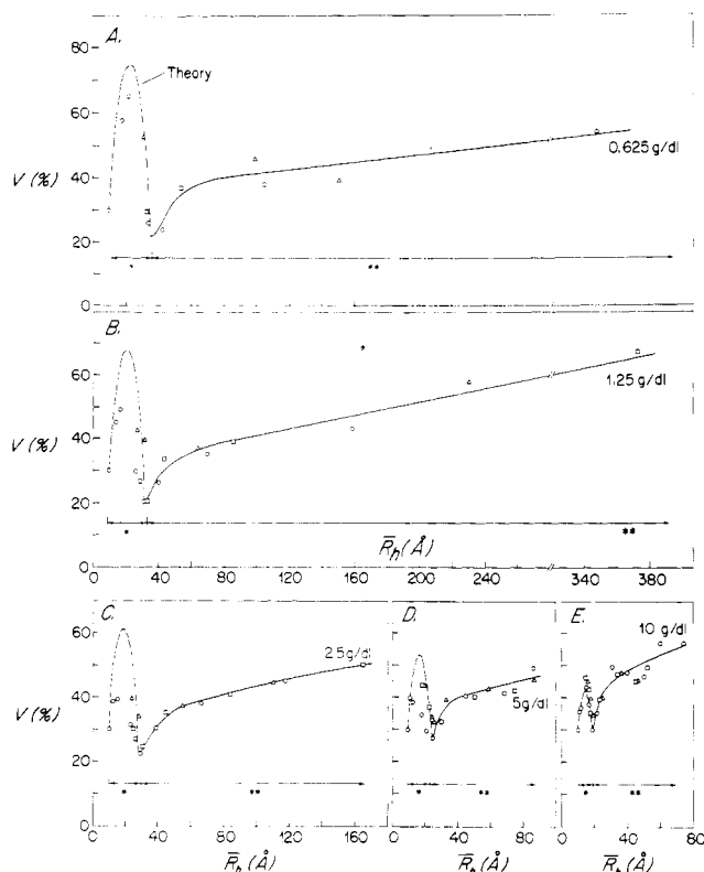
FIGURE 5: (A-E) Index of polydispersity, V , plotted vs. the corresponding R_h values measured in TC-L solutions at various temperatures [(O) 20; ( \square ) 40; ( \Delta ) 60 °C] and total lipid concentrations: (A) 0.625; (B) 1.25; (C) 2.5; (D) 5; (E) 10 g/dL. At low R_h values, simple and mixed micelles coexist, as shown by the horizontal arrows marked (*), and theoretical predictions (dashed curves) are shown for the dependence of V on R_h expected in these regions. At high R_h values, only mixed micelles are present as shown by the horizontal arrows marked (**). (See the text for further explanation.)
