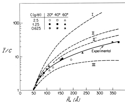
FIGURE 7: Experimental and theoretical dependence of the reduced intensity ( \bar{I}/C ) on the mean hydrodynamic radius, \bar{R}_h , of the micelles. Data are derived from a total lipid concentration of 0.625–2.5 g/dL at 20, 40, and 60 °C (see the key). Theoretical curves represent different mixed micellar shapes: I, monodisperse spheres; II, monodisperse disks (thickness 50 Å); III, monodisperse rods (diameter 50 Å). Curve II' represents calculations for polydisperse disks (Appendix B) and is in closest agreement with the experimental data (solid line).
