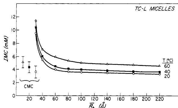
FIGURE 15: Dependence of IMC (mM) on \bar{R}_h for TC-L mixed micelles at ( \circ ) 20, ( \blacksquare ) 40, and ( \Delta ) 60 °C, as derived from parts A, B, and C of Figure 14. Note also the vertical bars representing (mean \pm SEM) estimates of the cmc of pure TC solutions at 20, 40, and 60 °C from Carey & Small (1969).
